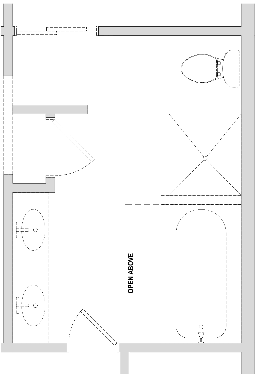
1. MASTER BATHROOM-DEMOLITION 1/2" = 1'-0"
