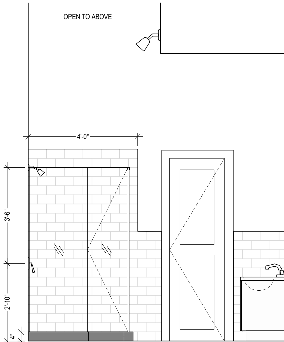
ELEVATION C 1/2" = 1'-0"
