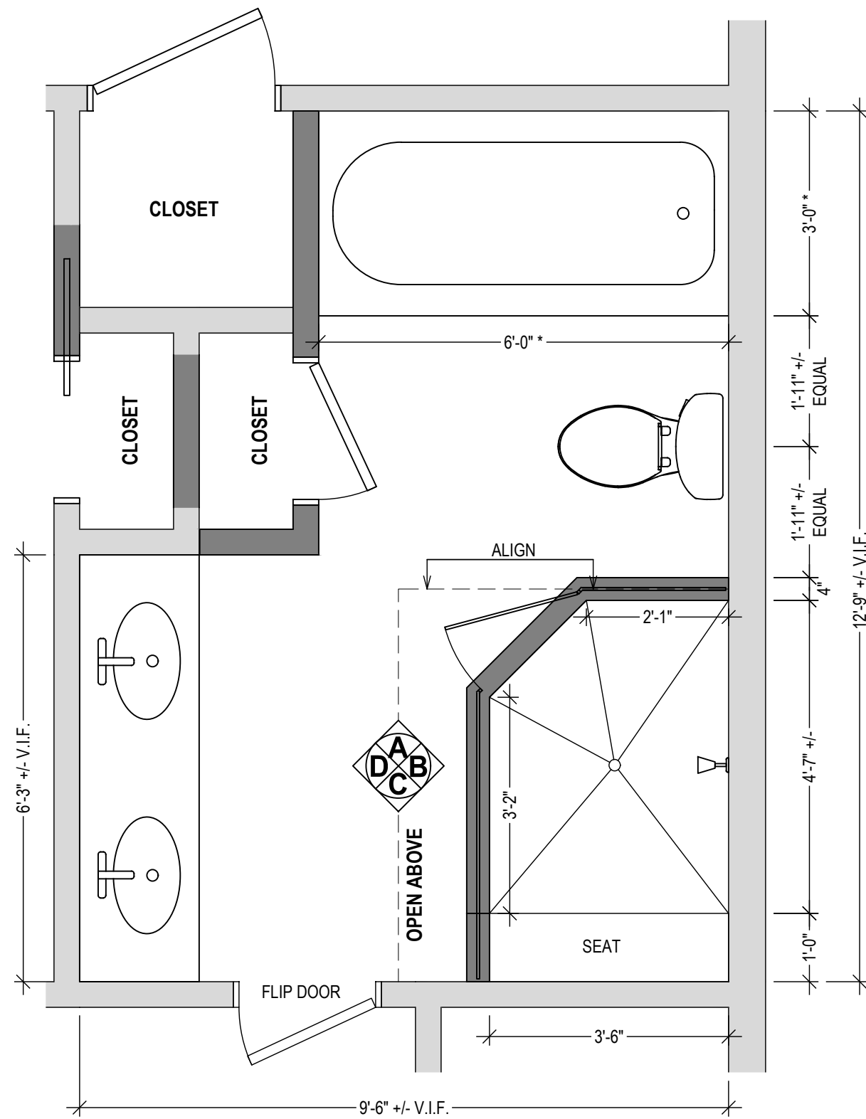
2. MASTER BATHROOM-PROPOSED 1/2" = 1'-0"
