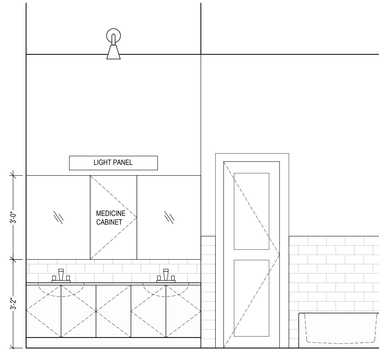
ELEVATION D 1/2" = 1'-0"
