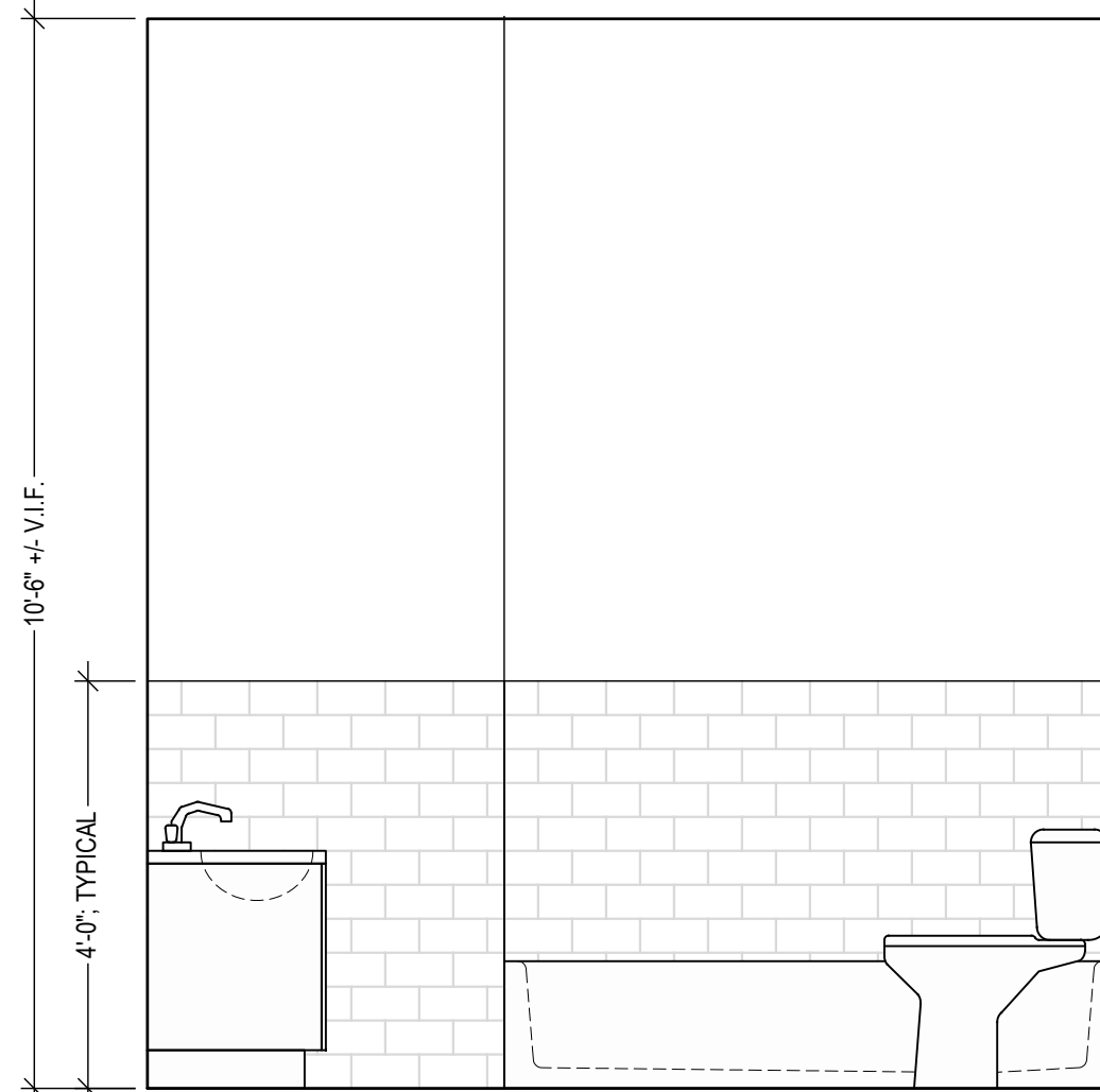
ELEVATION A 1/2" = 1'-0"
