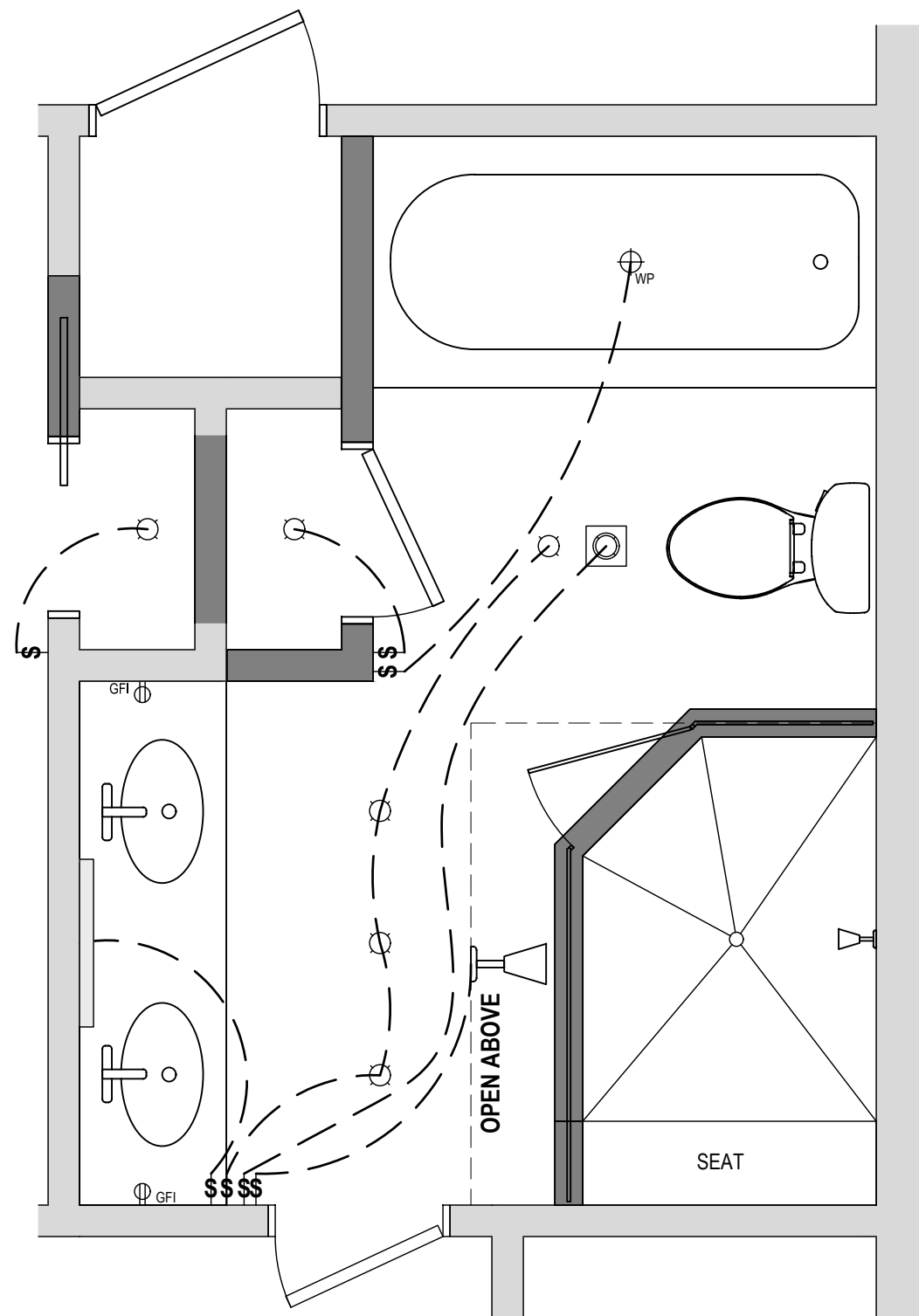
3. MASTER BATHROOM-ELECTRICAL 1/2" = 1'-0"
