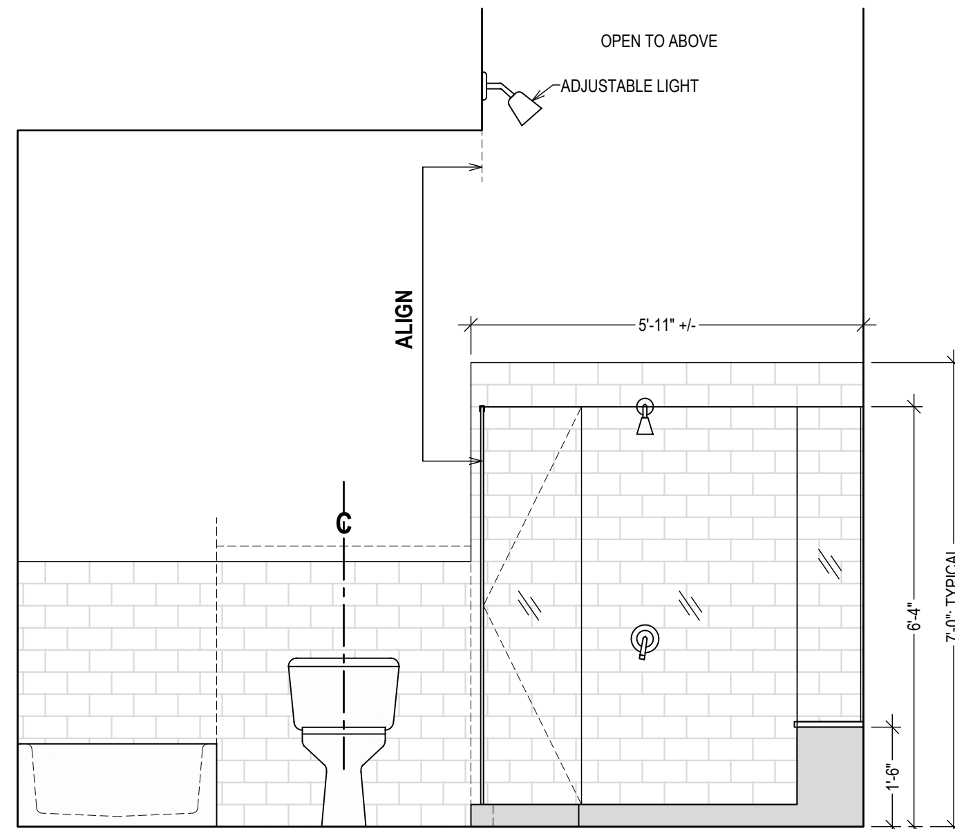
ELEVATION B 1/2" = 1'-0"
